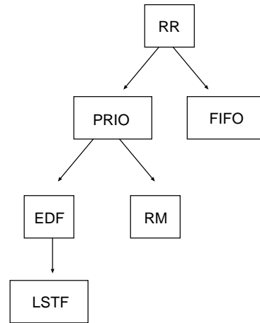
Figure 4: Inheritance Graph for Schedulers
